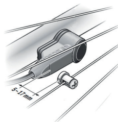
Image 31: Distance between the speed sensor and the speed sensor magnet
